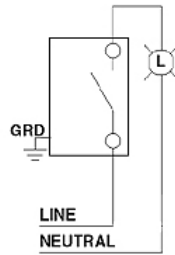
Wiring Diagram Single Pole
